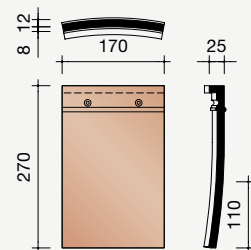
P3018900 Bolle pan (Napoleonschoed)
